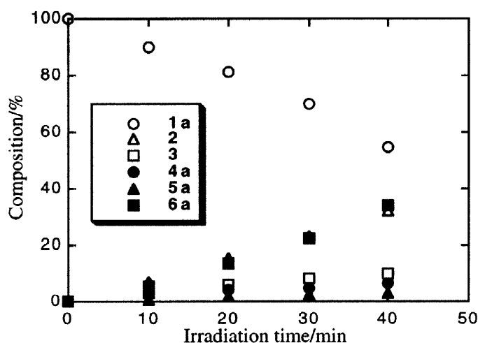
Figure 1. Relation between irradiation time and composition of each compound in methanol.
