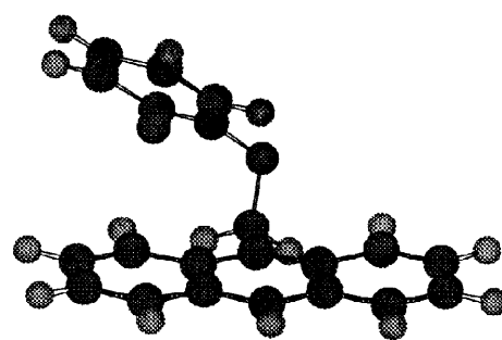
Figure 2. Energy-minimized conformation of 1a .
