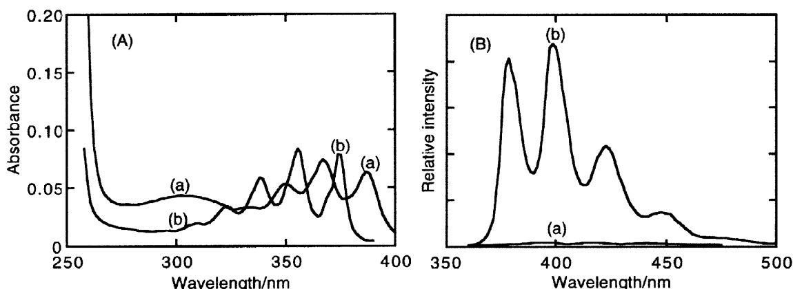
Figure 3. UV absorption (A) and fluorescence (B; \lambda_{ex} = 342 nm) spectra of 1a (curve a; 0.7 \times 10^{-5} mol dm ^{-3} ) and anthracene (curve b; 1.0 \times 10^{-5} mol dm ^{-3} ) in methanol at room temperature.
